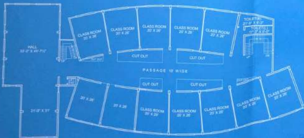
SECOND FLOOR PLAN ( BLOCK-A )
